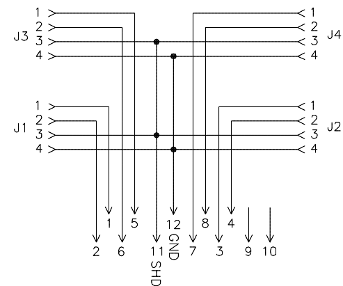
P1 WIRING DIAGRAM
